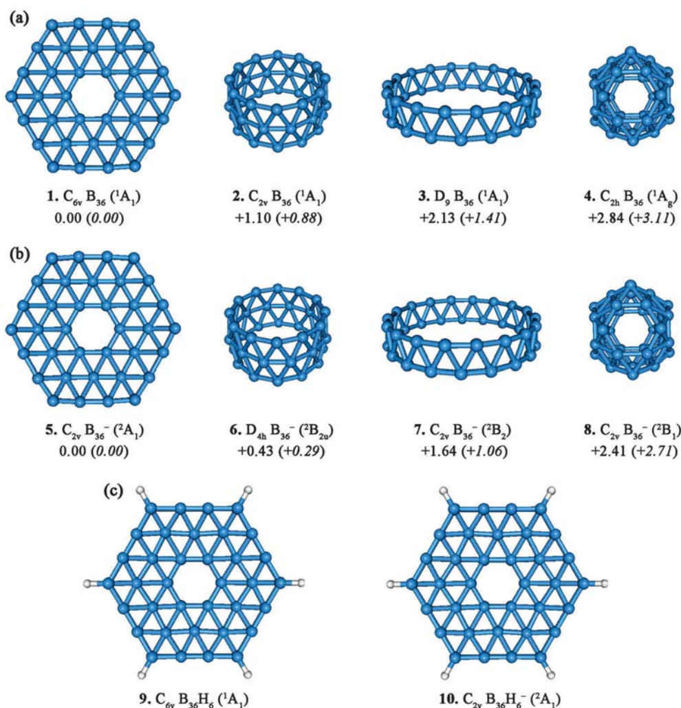
Fig. 1 Selected optimized structures at the PBE0/6-311+G* level for B_{36} ( 1–4 ), B_{36}^- ( 5–8 ), and their hydrogenated clusters B_{36}H_6 ( 9 ) and B_{36}H_6^- ( 10 ). The B_{36} ( 1 ) and B_{36}^- ( 5 ) structures are established as the global minima. Relative energies are shown in eV at the PBE0 and TPSSh (in italic ) levels.
