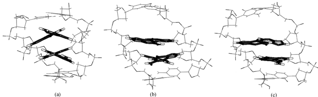
Fig. 3. (a) Sheared mismatch; (b) and (c) conformation of mismatched base pairs after repair for L -isomer and D -isomer.
