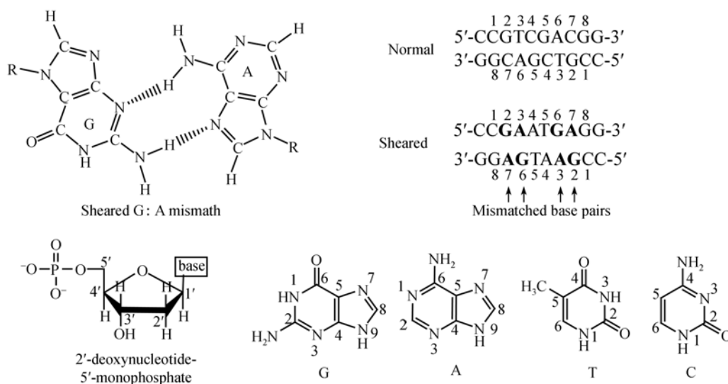
Fig. 2. Sheared G: A mismatch and the DNA sequence studied in this work.
