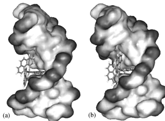
Fig. 6. The complex ((a) L -isomer and (b) D -isomer) entered the hydrophobe cavity from major groove orientation.
