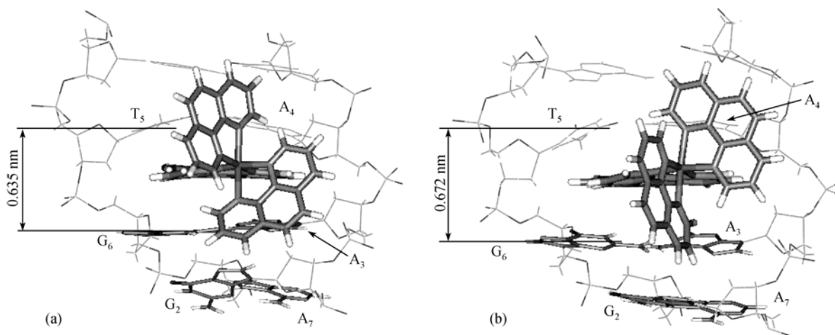
Fig. 7. The structure of L -isomer-DNA association (a) and that of D -isomer-DNA association (b).
