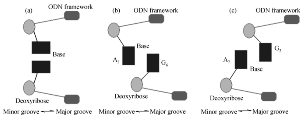
Fig. 5. (a) The arrangement of normal bases. (b) and (c), the arrangement of mismatched bases for G_6:A_3 and A_7:G_2 bases pairs.
