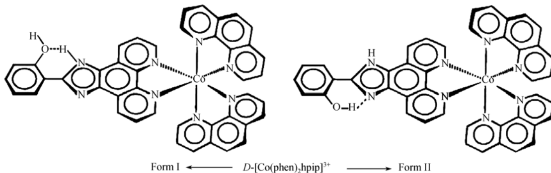
Fig. 1. Two forms of the complex. Form II was studied in this work.
