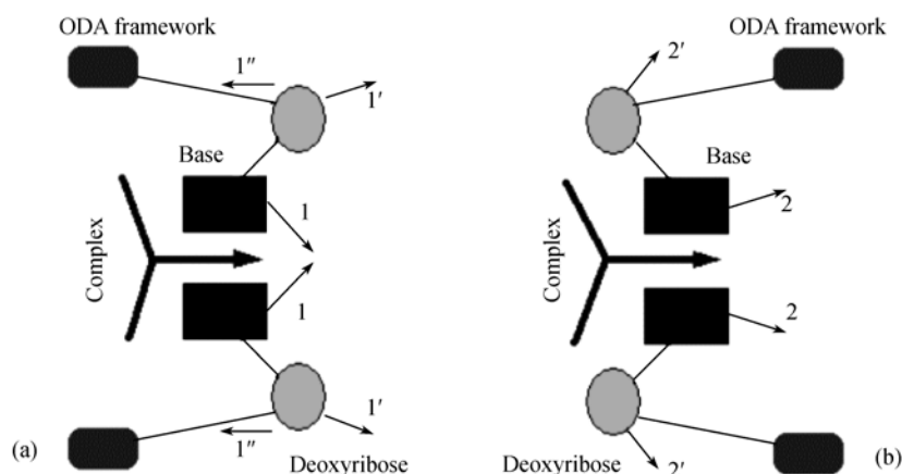
Fig. 4. The sketch map of steric hindrance. (a) Intercalation from the major groove, (b) intercalation from the minor groove.
